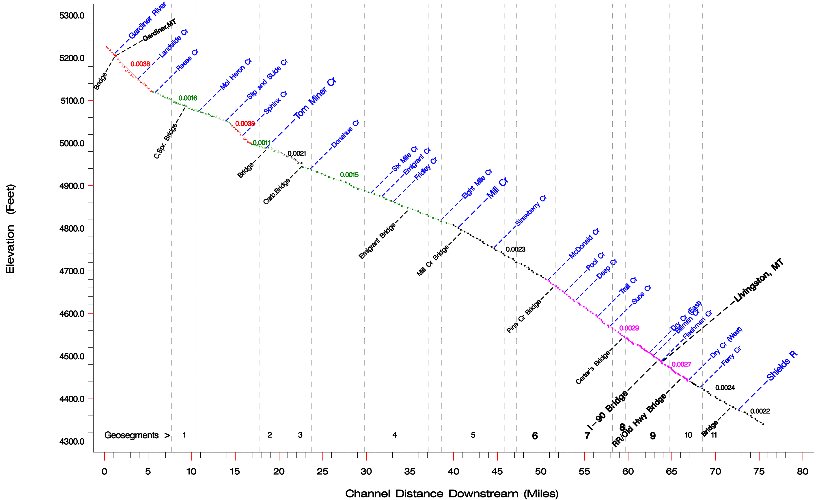
Figure 3. Yellowstone River Channel Profile: Gardiner, MT to Confluence with Shields River Water-surface profile on 4-11-1999 at discharge of 1500 cfs near Livingston, MT PRELIMINARY DATA SUBJECT TO REVISION -- November 2002
