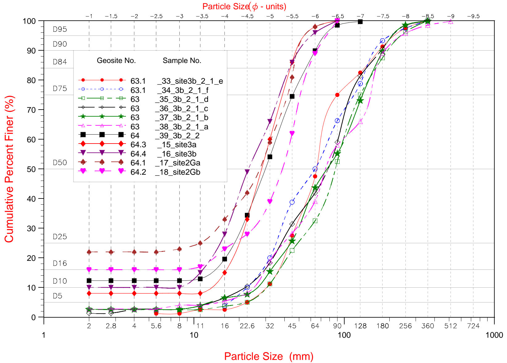
Figure 2b. Upper Yellowstone River Particle-Size Distribution: Surface Samples Geosites 63 to 64.2 -- Located between 9th St Bridge and RR Bridge
