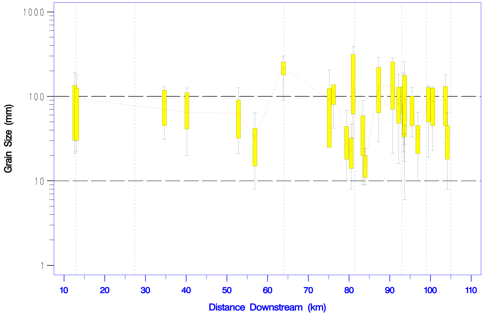
Figure 2a. Particle-Size Distribution: Selected Sites Upper Yellowstone River Corwin Springs to Livingston, MT (Upstream end of alternate bars and point bars)
