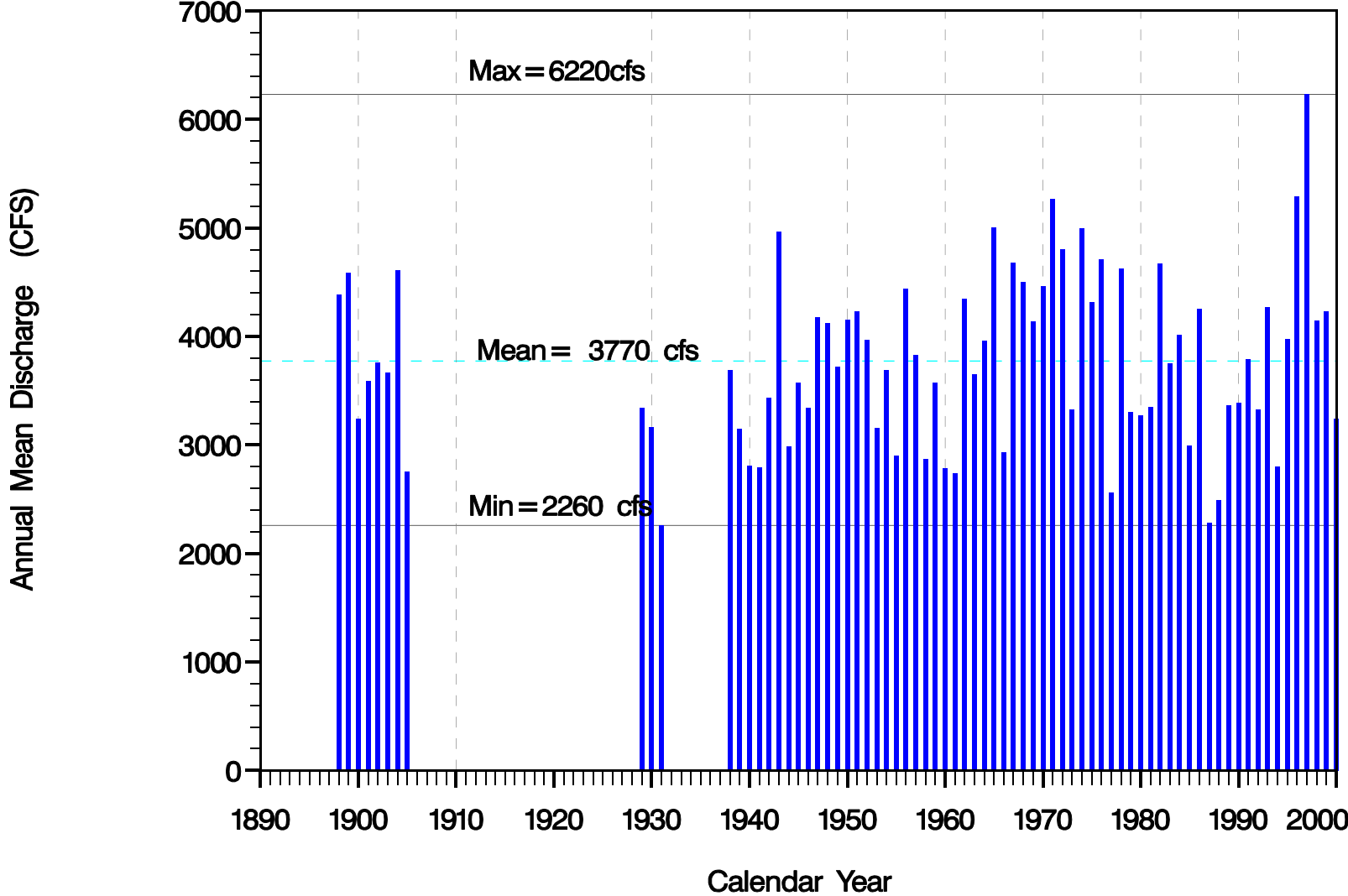
Figure 23 Average Annual Runoff: Yellowstone River near Livingston, MT (Carters Bridge) 1897 – 2000
